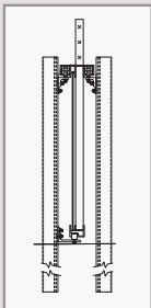
Track & Trolley Assembly (Double)
