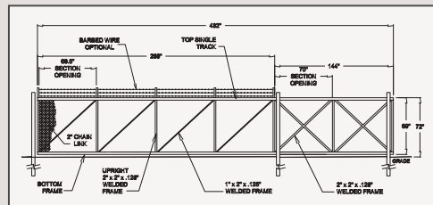
Chain Link Cantilever Gate (Detailed Example)
